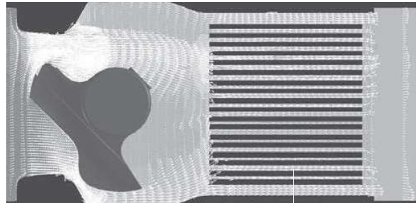
Cavitation breaker
